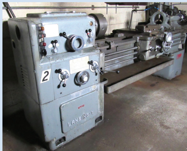
Lansing-T 16"/>" x 60" Geared-Head Gap Lathe
