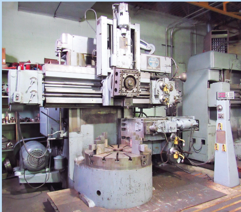
Bullard Man-Au-Trol 42" Vertical Turret Lathe
