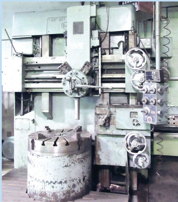
Bullard Model 75 36" Cutmaster Vertical Turret Lathe
