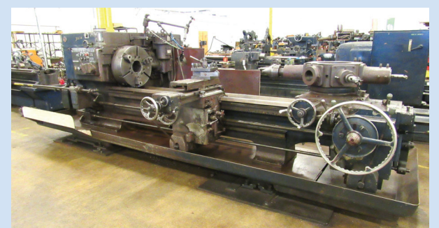
Warner & Swasey Model 3A Universal Saddle-Type, Cross-Sliding Turret Lathe
