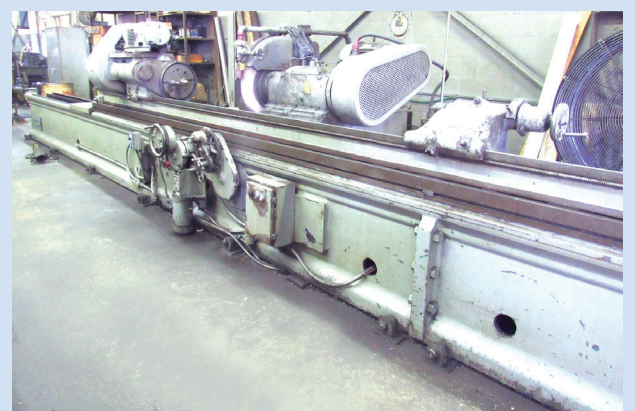
Norton 14" x 188" Plain Hydraulic Cylindrical Grinder
