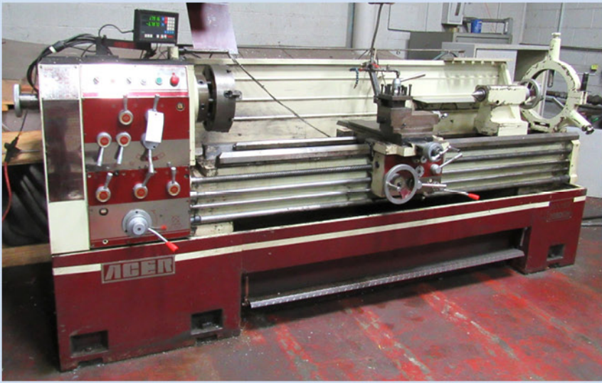
ACER DYNAMIC 2080GH 20"/27.5" x 80" GEARED HEAD LATHE
