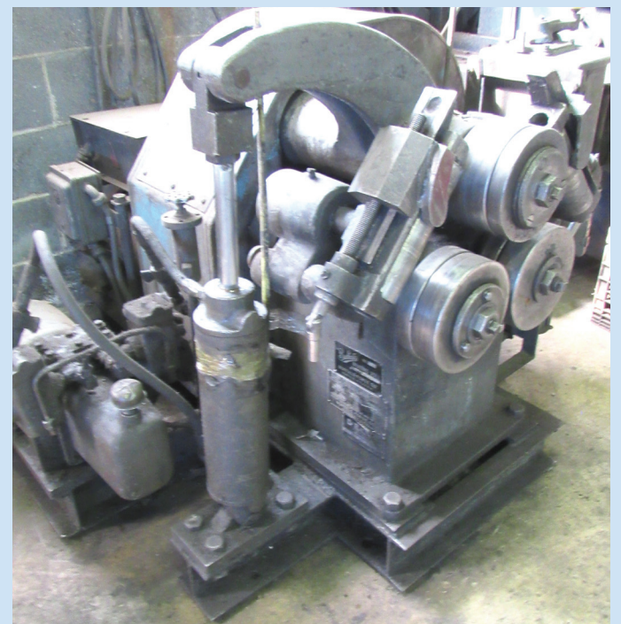
BUFFALO No. 1/2 2" x 2" x 1/4" Angle Bending Roll
