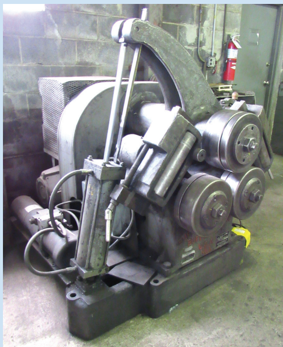
BUFFALO No. 1VBR 3" x 3" x 3/8" Angle Bending Roll
