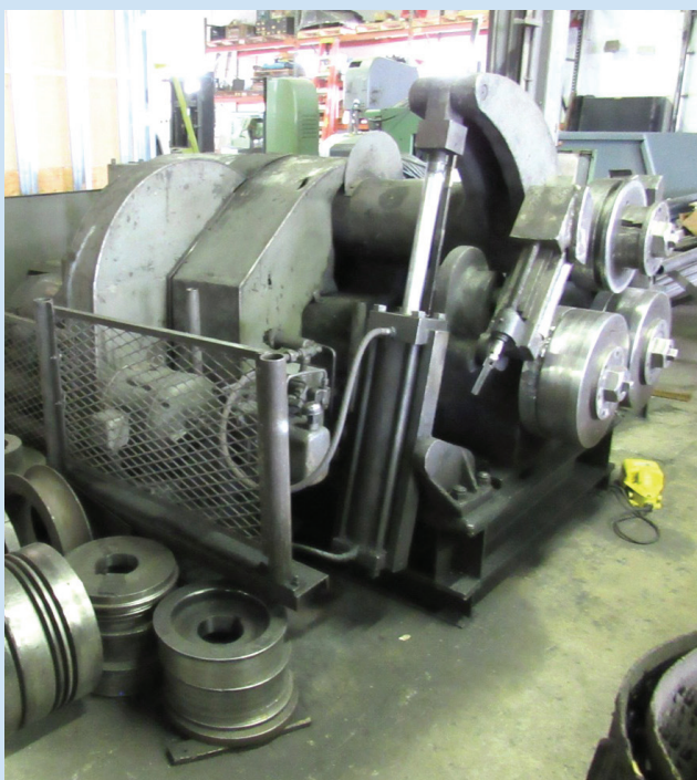
BUFFALO No. 2 5" x 5" x 3/8" Angle Bending Roll
