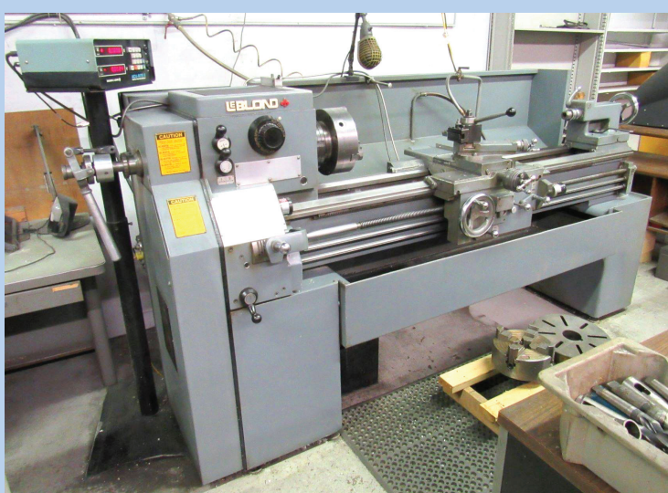
LeBlond Servo-Shift 15" x 54" Geared Lathe
