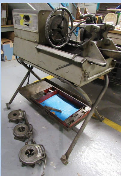
Oster Model 552 Pipe Threading Machine
