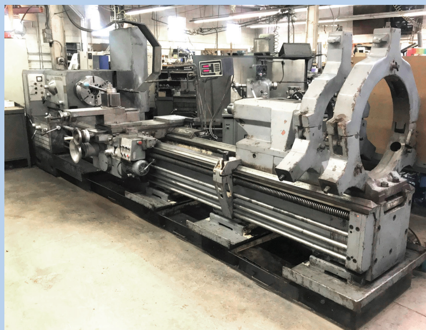
Poreba Model TR-80BIS 32"/43" x 120" Geared Lathe
