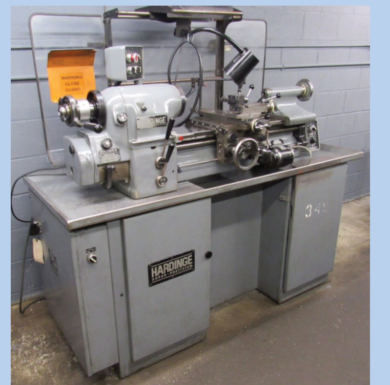
HARDINGE "Super Precision" HLV-H Precision Toolroom Lathe
